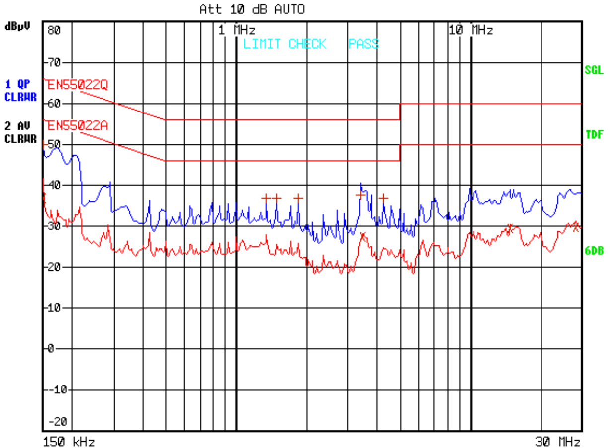
Figure 79 – 115 VAC, 100% Load.
